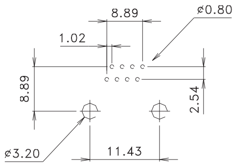
PCB LAYOUT
