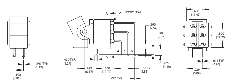
ER8011L - R11-2-Q Please see page B6 to know more about ER812L (3-way Switches)
