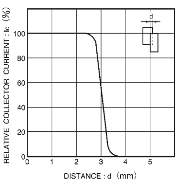
Fig.6 Relative output vs. distance characteristics
