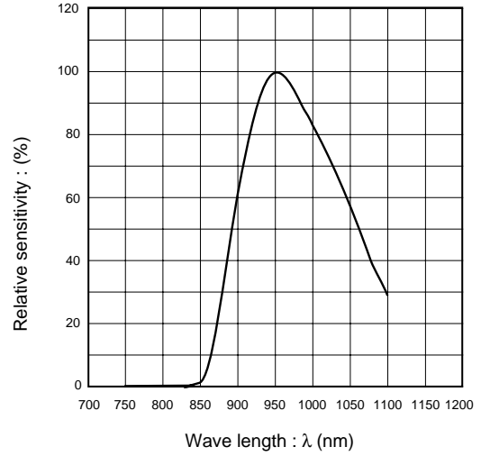
Fig.7 Relative spectral sensitivity of photo diode
