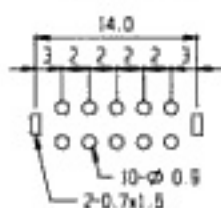
PCB LAYOUT
