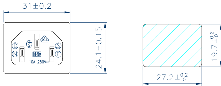
PANEL CUTOUT
