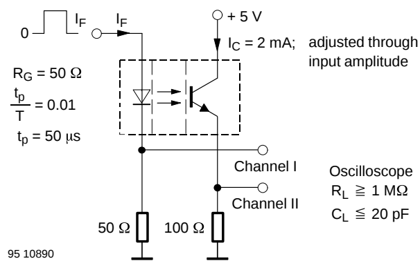
Figure 1. Test circuit
