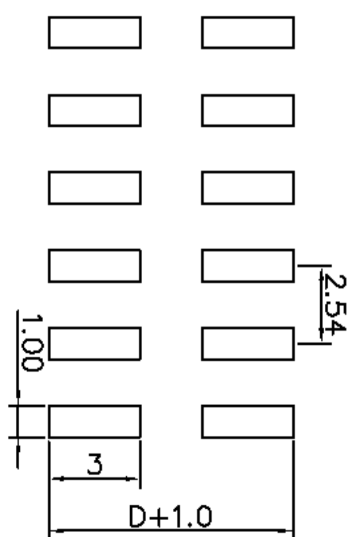
PCB Layout
