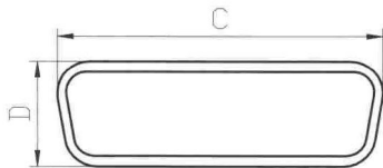
母型连接器插合位外部尺寸 Outer size of female mating location
