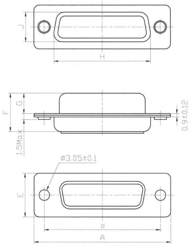
母型连接器插合位外部尺寸 Outer size of female mating location
